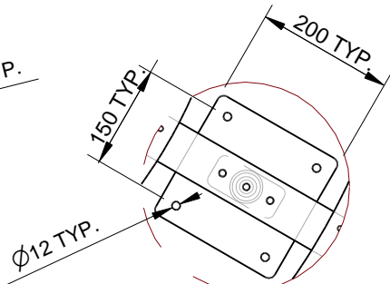
Detail B BENCH BOLT DOWN DETAIL TIMBER SLATS REMOVED FOR CLARRITY
