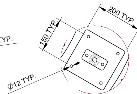
Detail B BENCH BOLT DOWN DETAIL TIMBER SLATS REMOVED FOR CLARRITY
