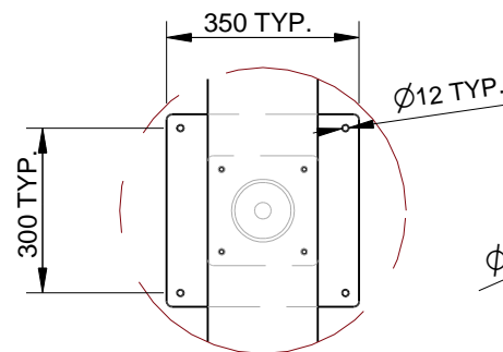
Detail A TABLE BOLT DOWN DETAIL TIMBER SLATS REMOVED FOR CLARRITY
