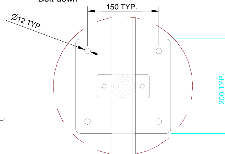
Detail A TYPICAL BOLT DOWN DETAIL TIMBER SLATS REMOVED FOR CLARRITY
