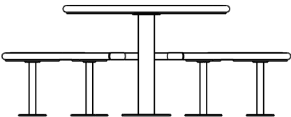
Detail A TABLE BOLT DOWN DETAIL TIMBER SLATS REMOVED FOR CLARRITY
