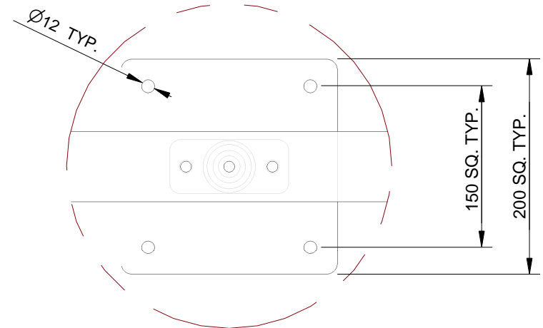
Detail A TYPICAL BOLT DOWN DETAIL TIMBER SLATS REMOVED FOR CLARRITY
