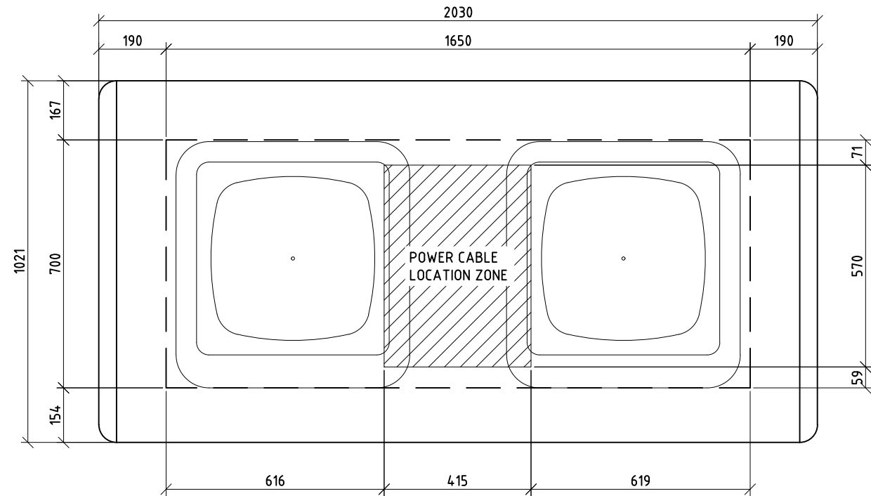
1 PLAN SCALE (1:15)
