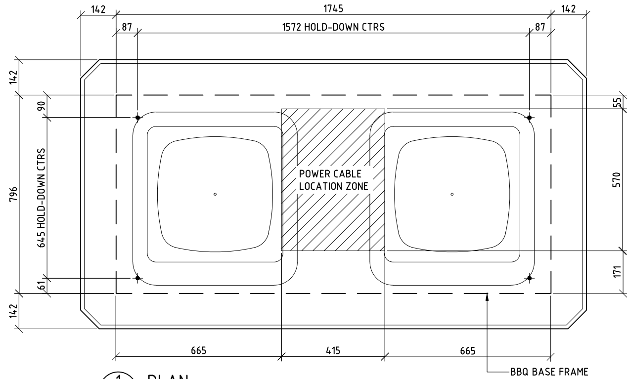
1 PLAN SCALE (1:15)
