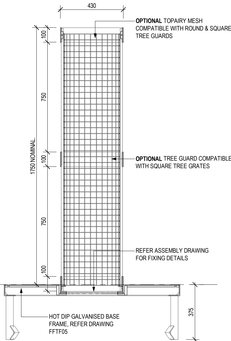
2 SECTIONAL VIEW
