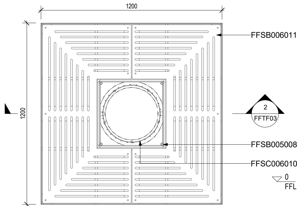
1 PLAN VIEW
