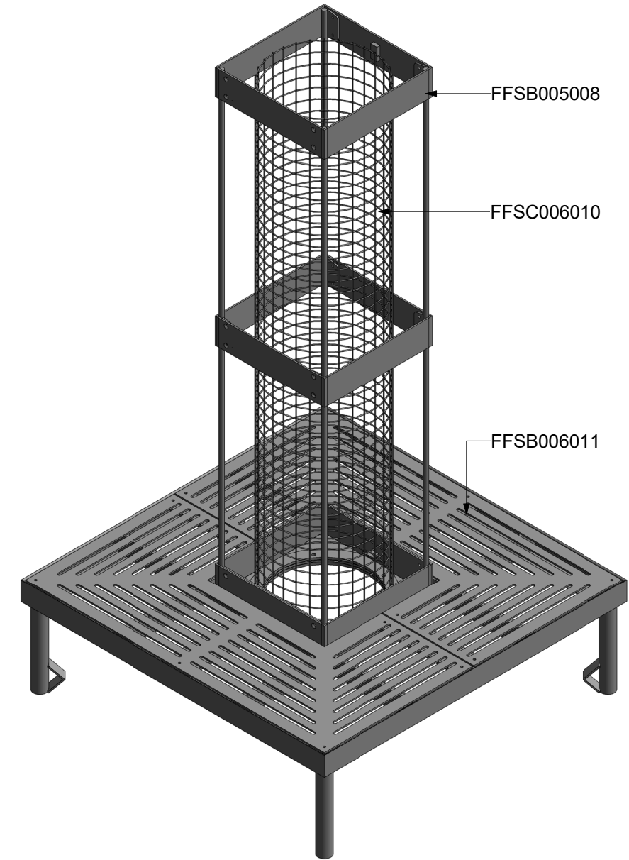
3 ISOMETRIC VIEW
