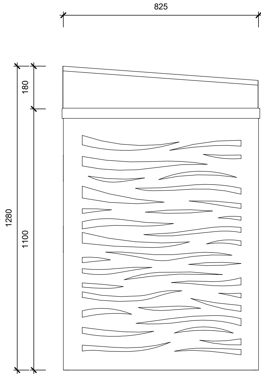
SIDE ELEVATION
