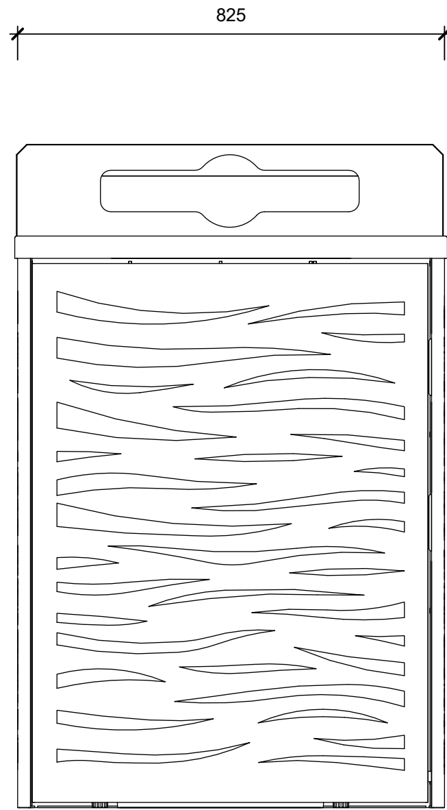
FRONT ELEVATION
