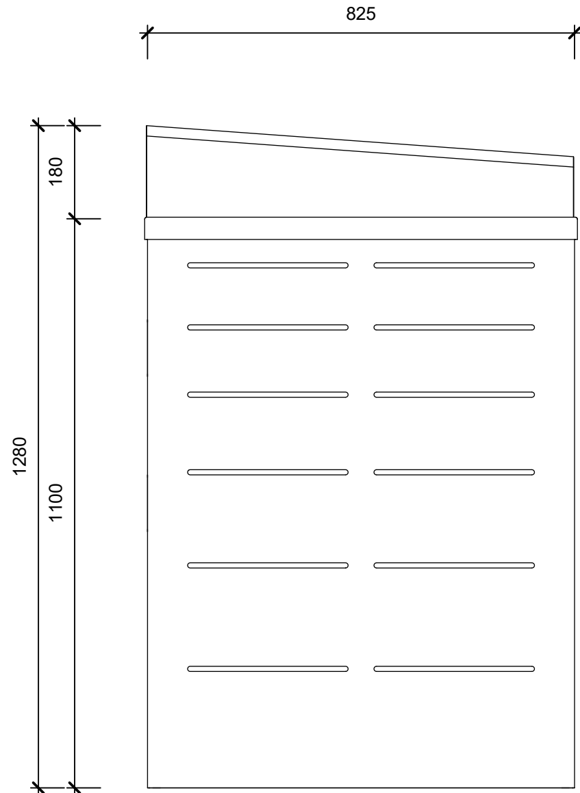
SIDE ELEVATION
