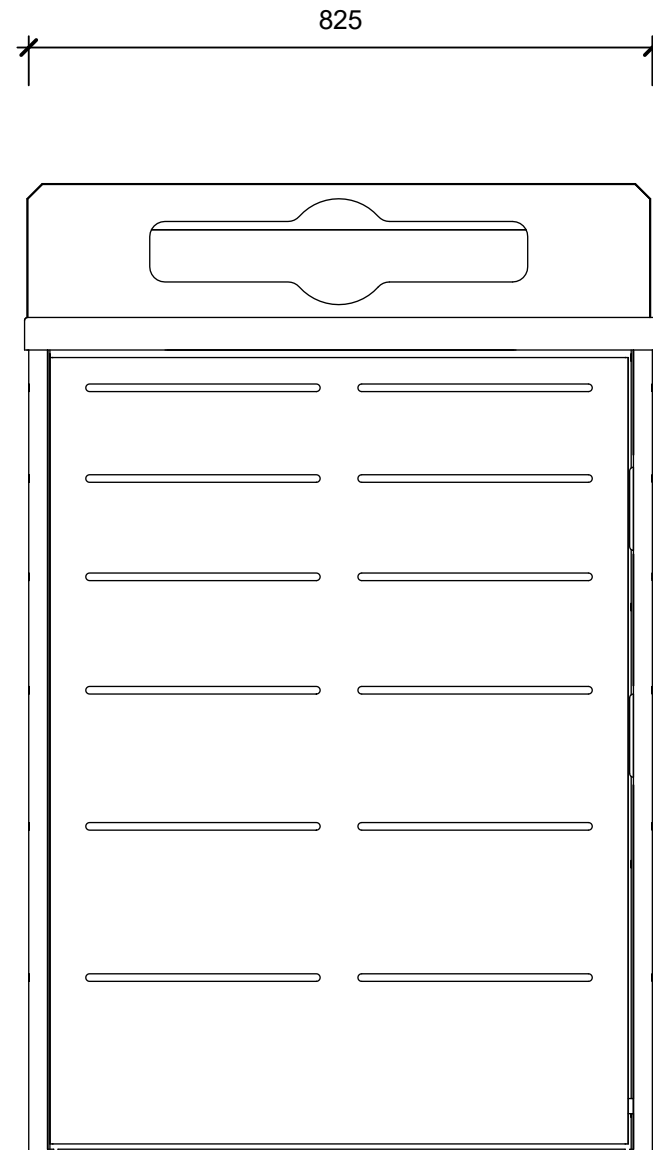
FRONT ELEVATION
