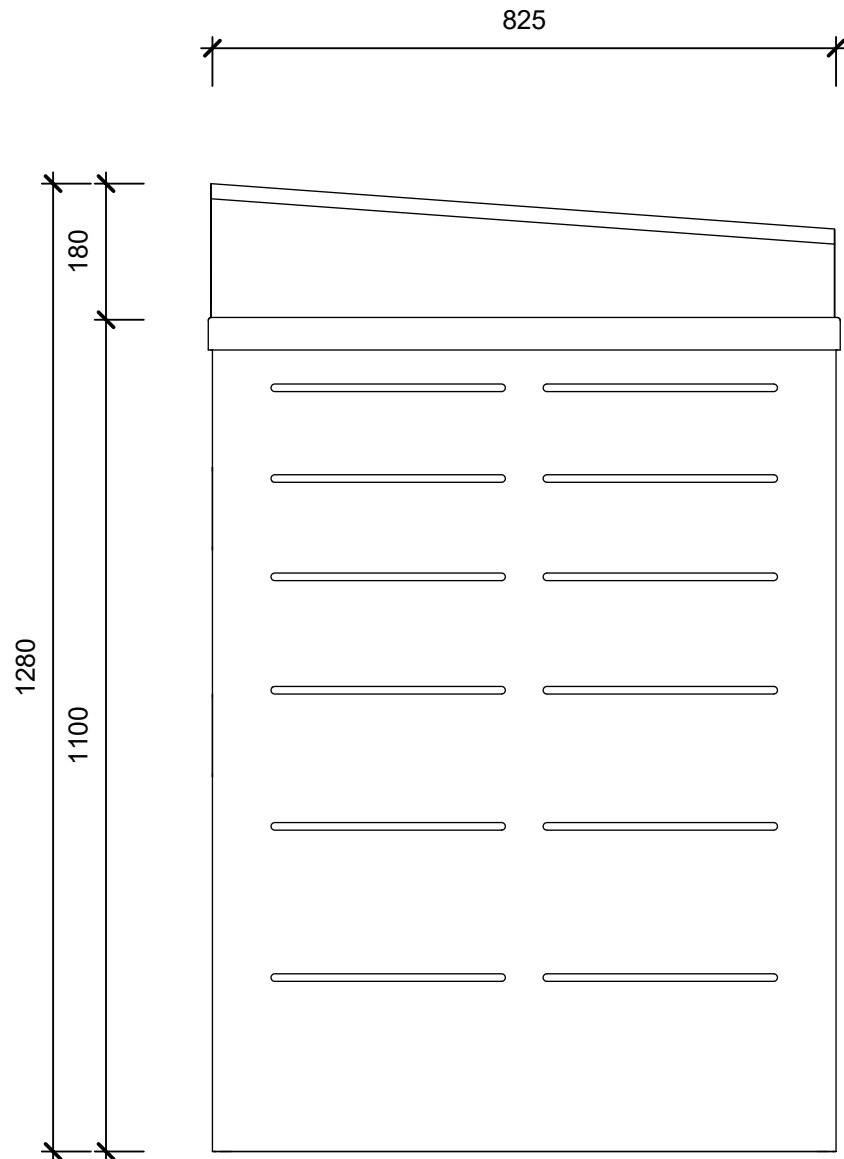
SIDE ELEVATION
