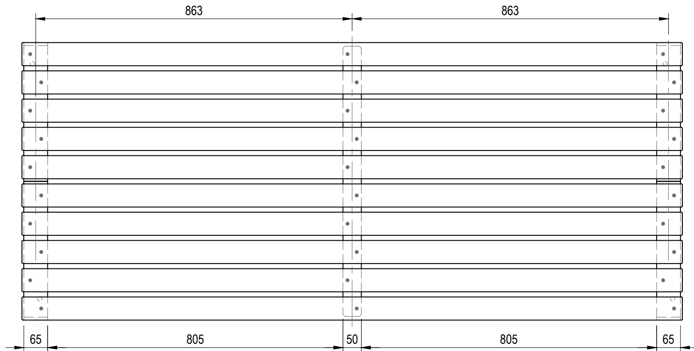
TOP VIEW
