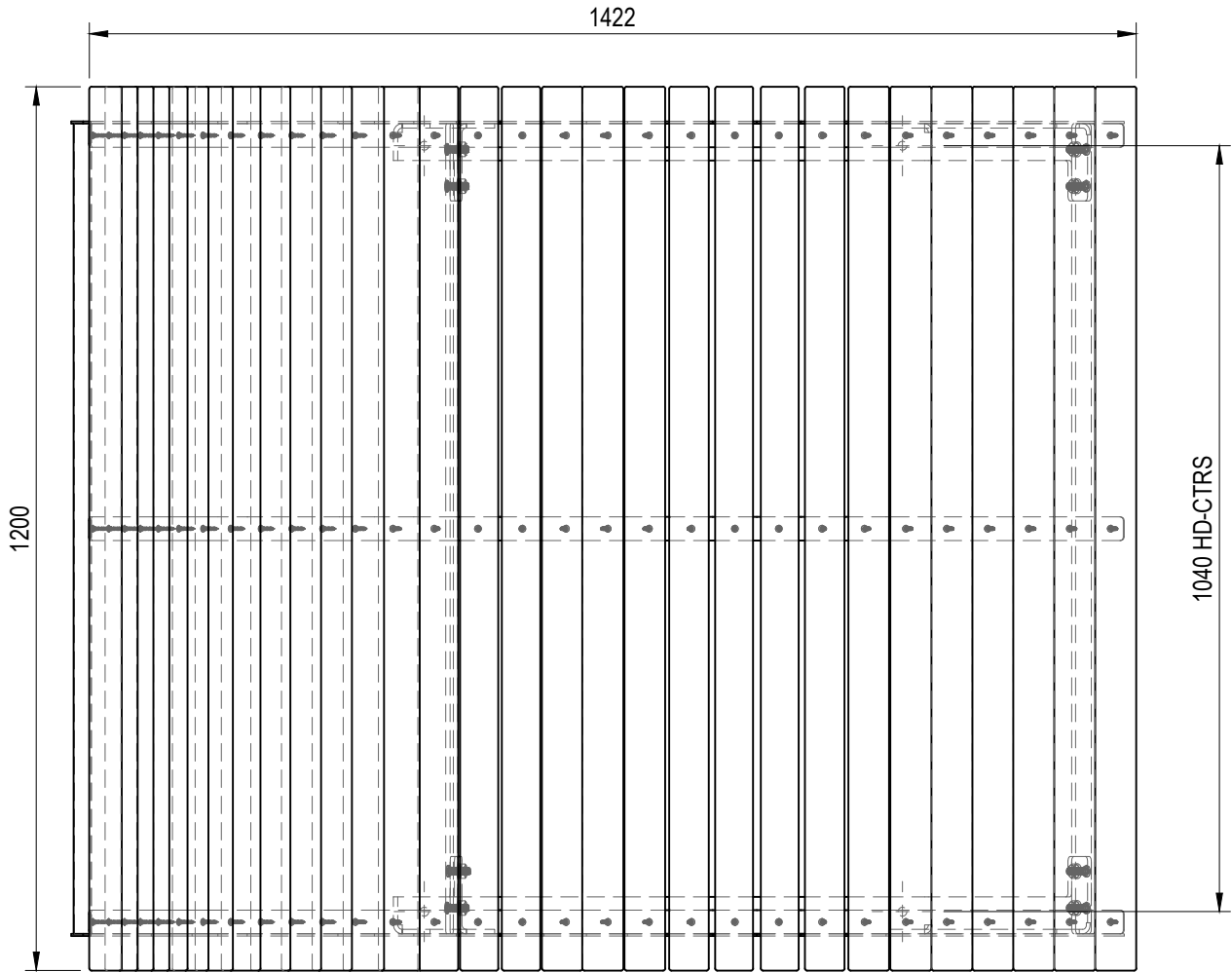
TOP VIEW
