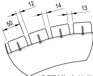
DETAIL-A (1:5)
