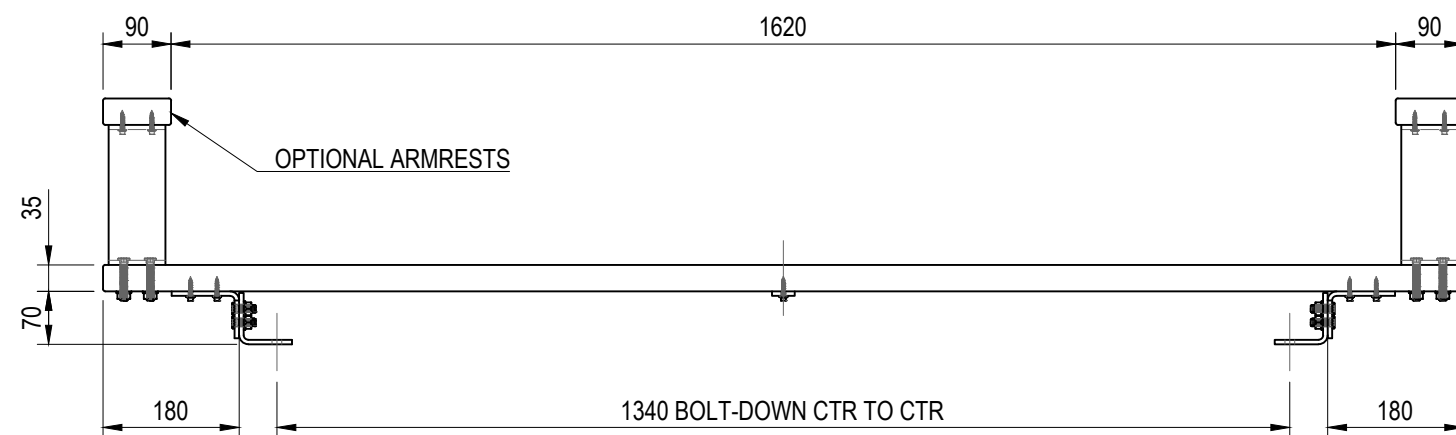
FRONT VIEW
