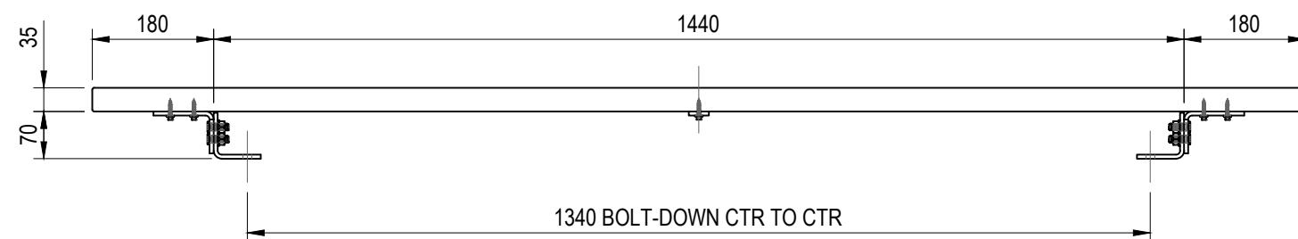
FRONT VIEW
