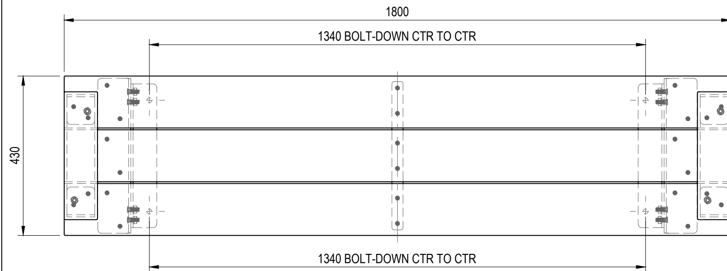
TOP VIEW
