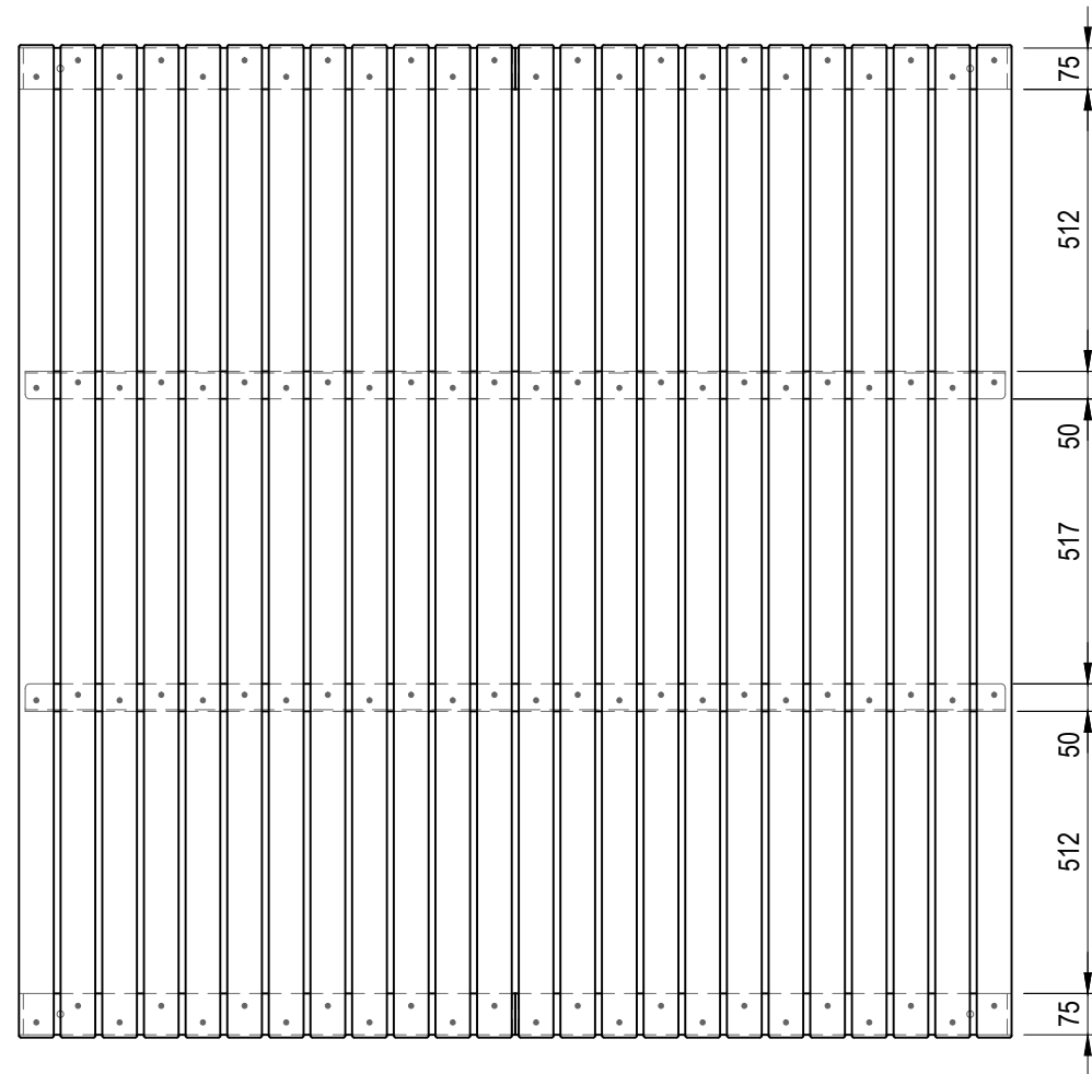
TOP VIEW
