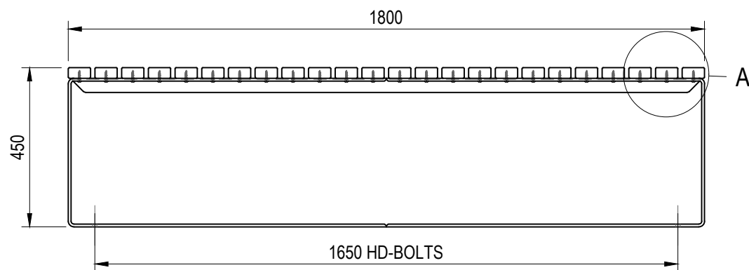
FRONT VIEW
