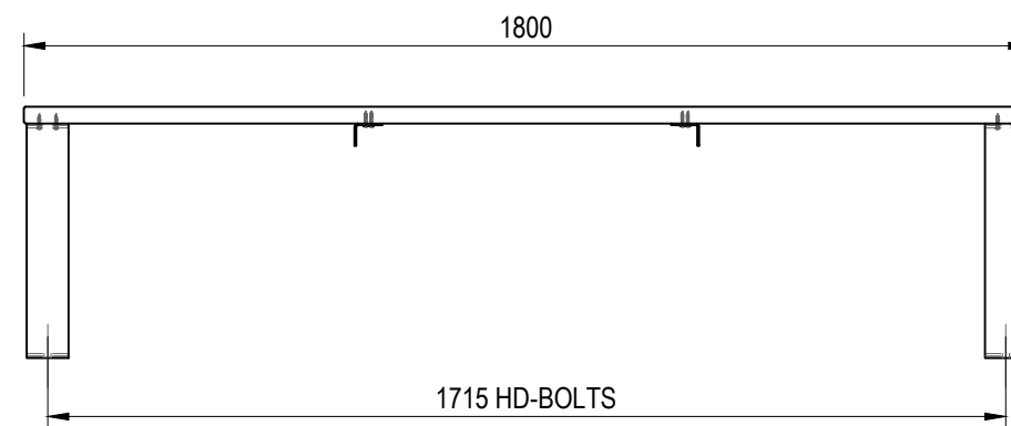
END VIEW
