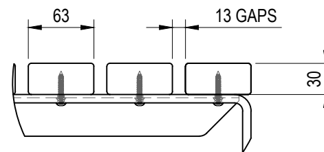
DETAIL A (1:5)
