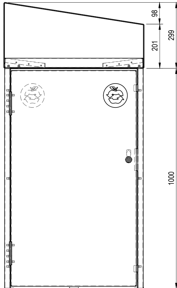
FRONT VIEW
