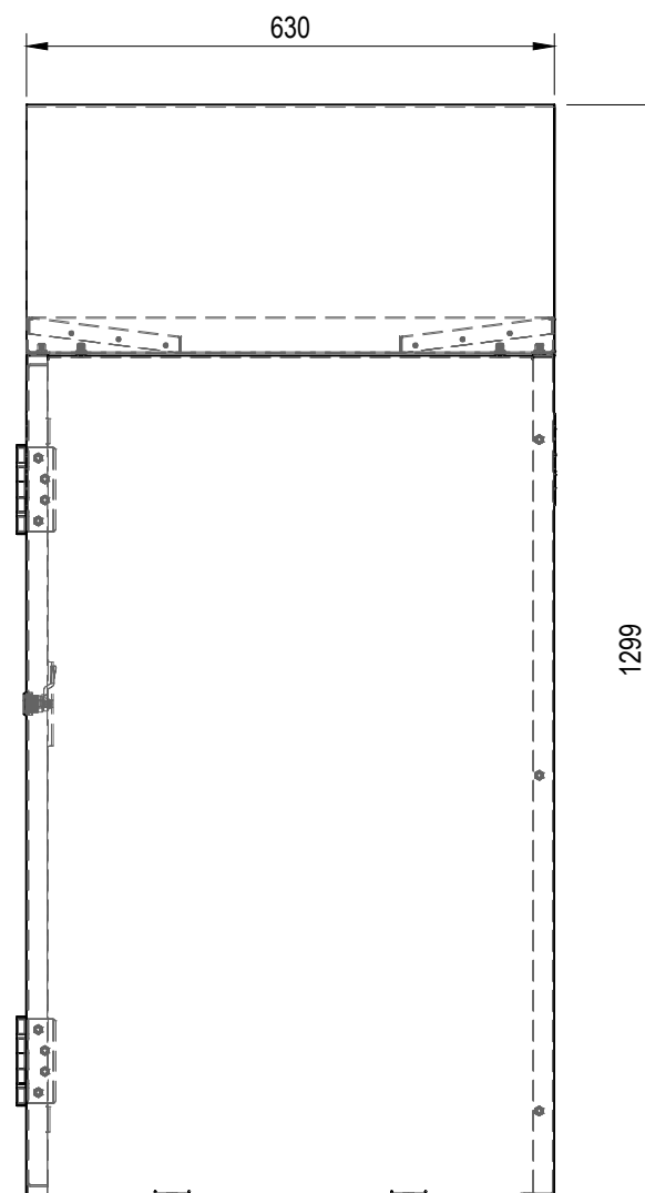
END VIEW
