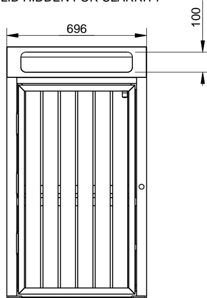
BOLT DOWN DETAIL LID HIDDEN FOR CLARRITY
