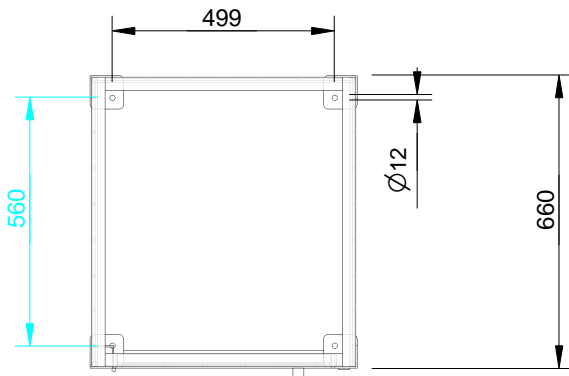
BOLT DOWN DETAIL LID HIDDEN FOR CLARRITY
