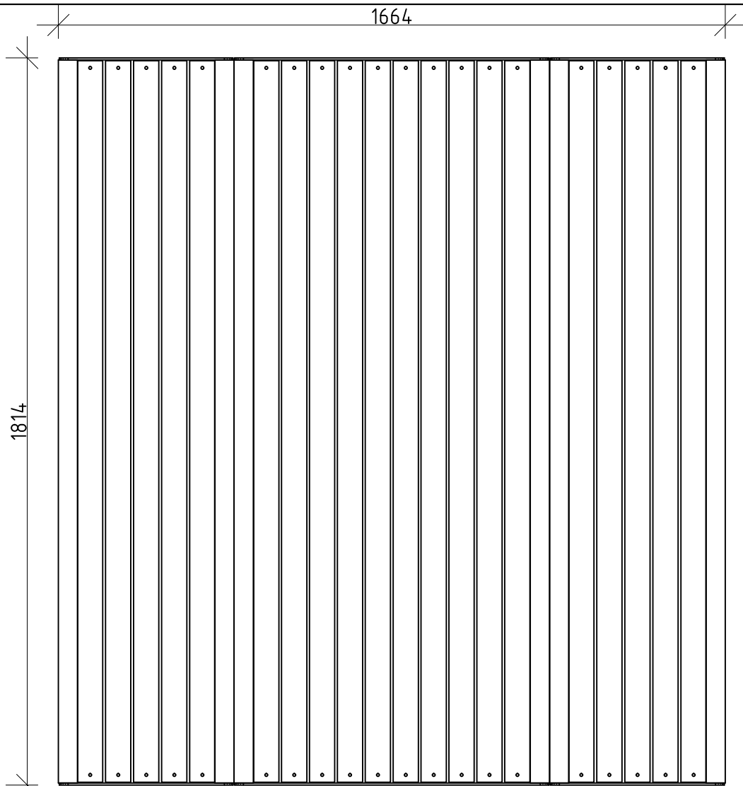
1 PLAN 1:15 @ A3
