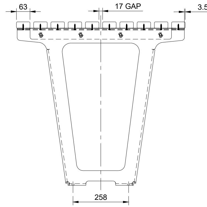
BD CENTRE TO CENTRE SIDE VIEW
