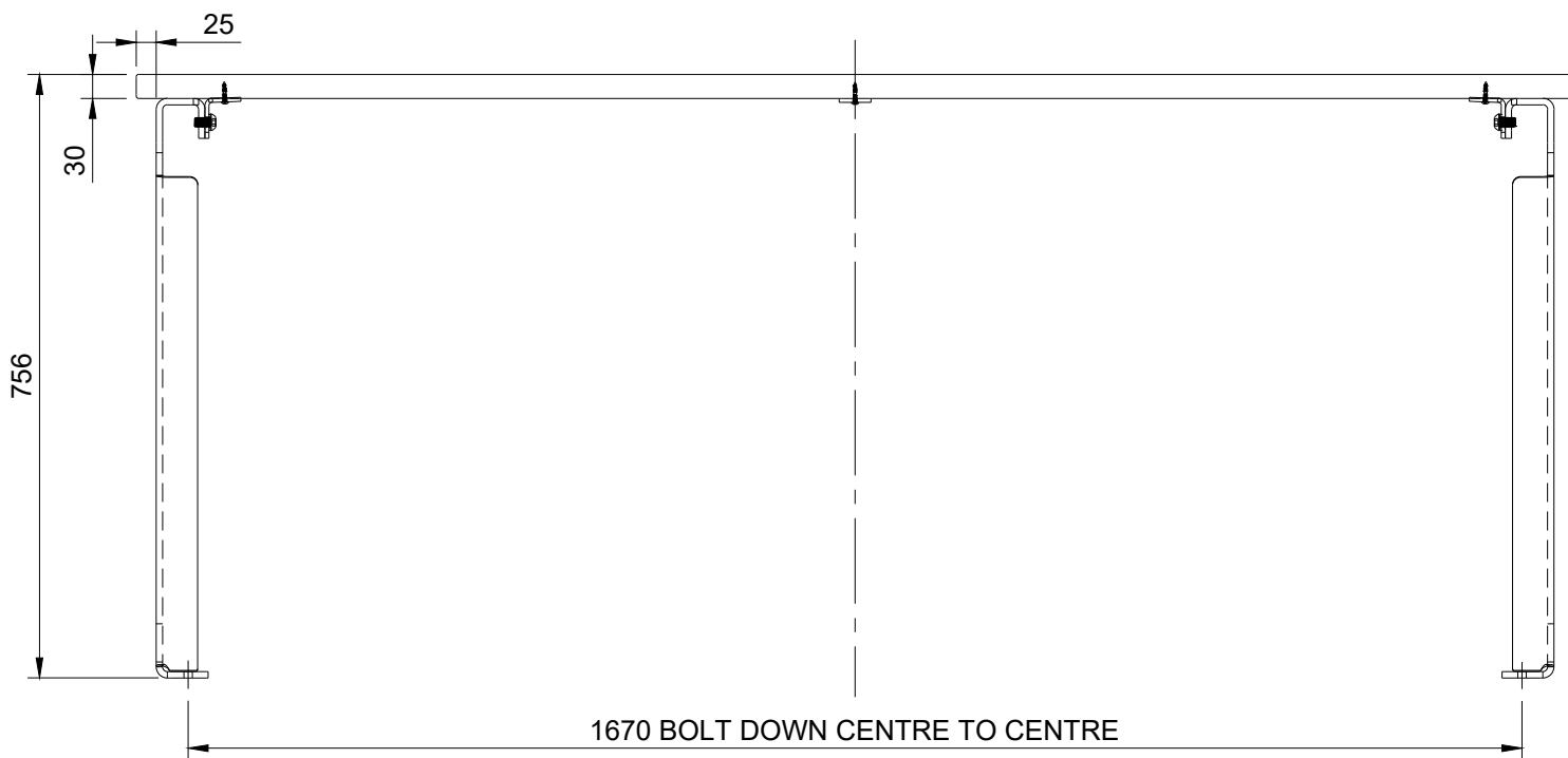
FRONT VIEW
