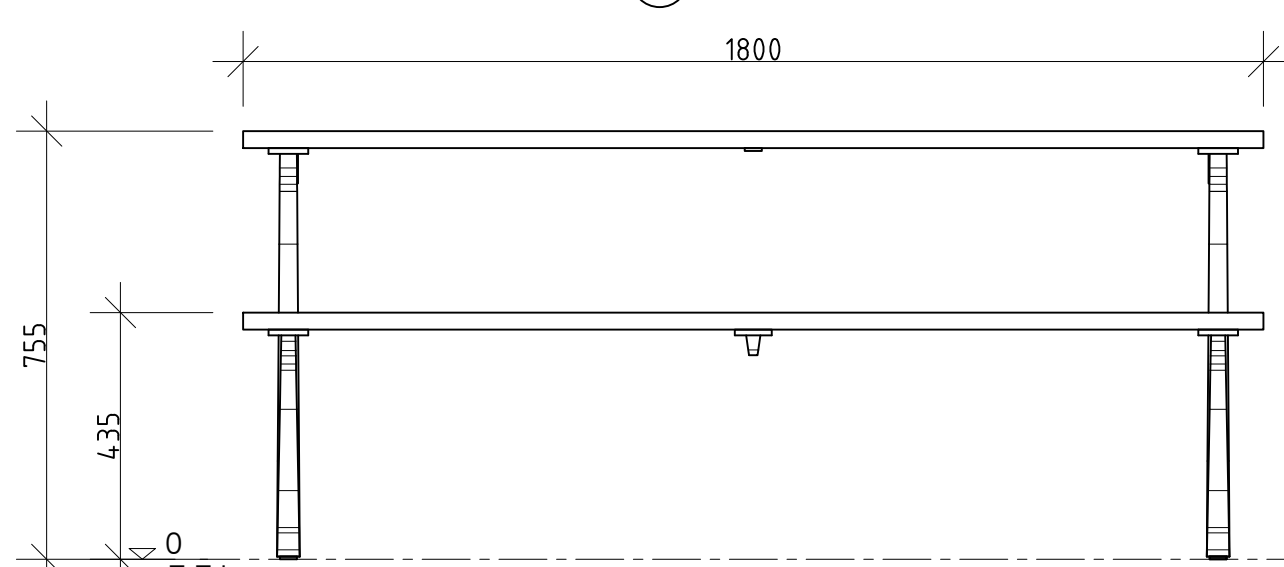
3 FRONT ELEVATION 1:15 @ A3
