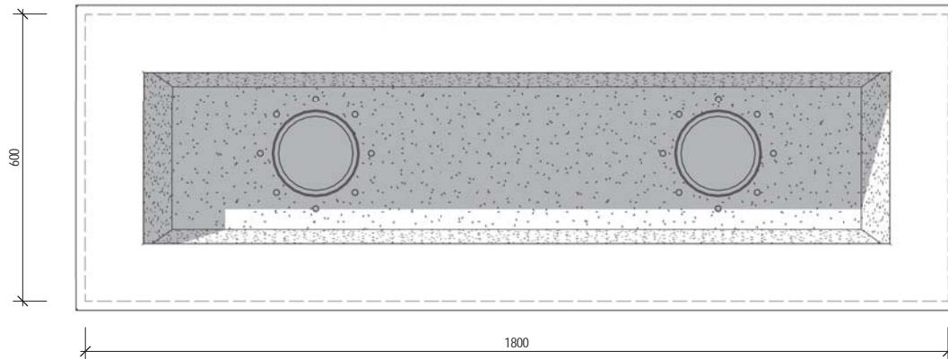
3 PLAN 001 1: 10 @ A3
