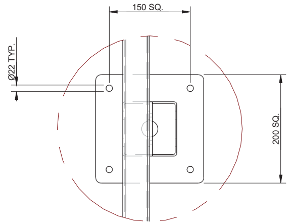
Detail A BOLT DOWN DETAIL ROOF HIDDEN FOR CLARRITY
