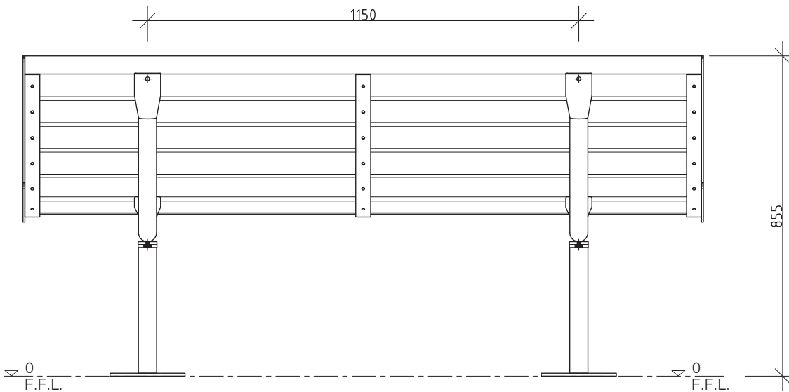
2 REAR ELEVATION 1:10 @ A3
