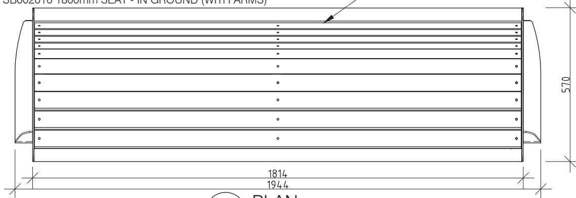
1 PLAN 1:10 @ A3
