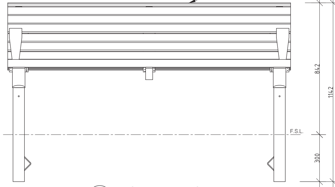
3 FRONT ELEVATION 1:10 @ A3
