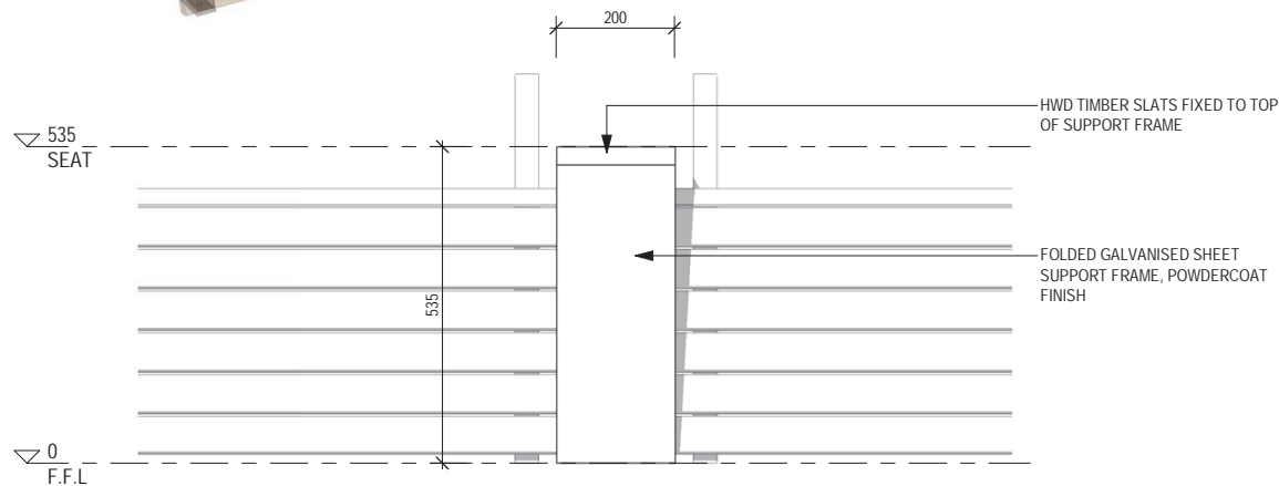
3 FRONT ELEVATION 1:10 @ A3
