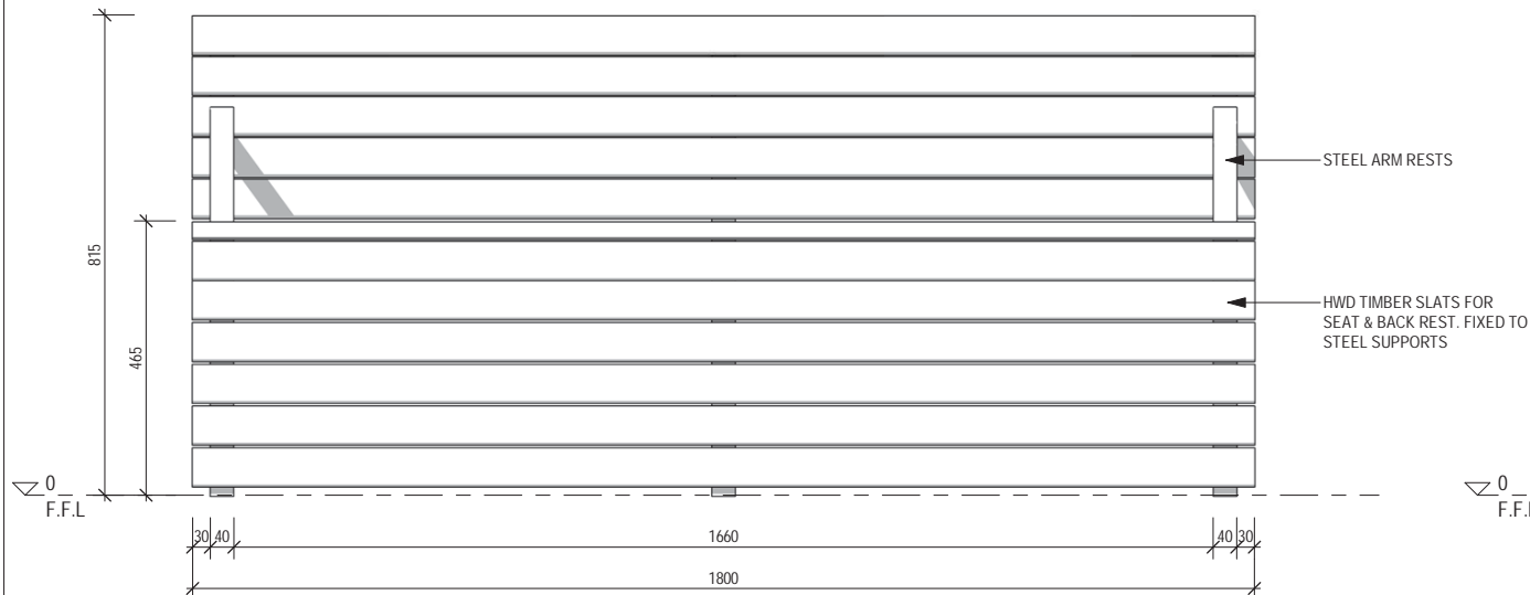
3 FRONT ELEVATION 1:10 @ A3
