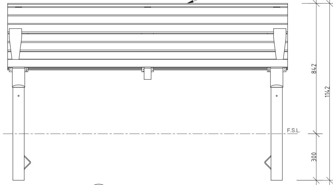
3 FRONT ELEVATION 1:10 @ A3
