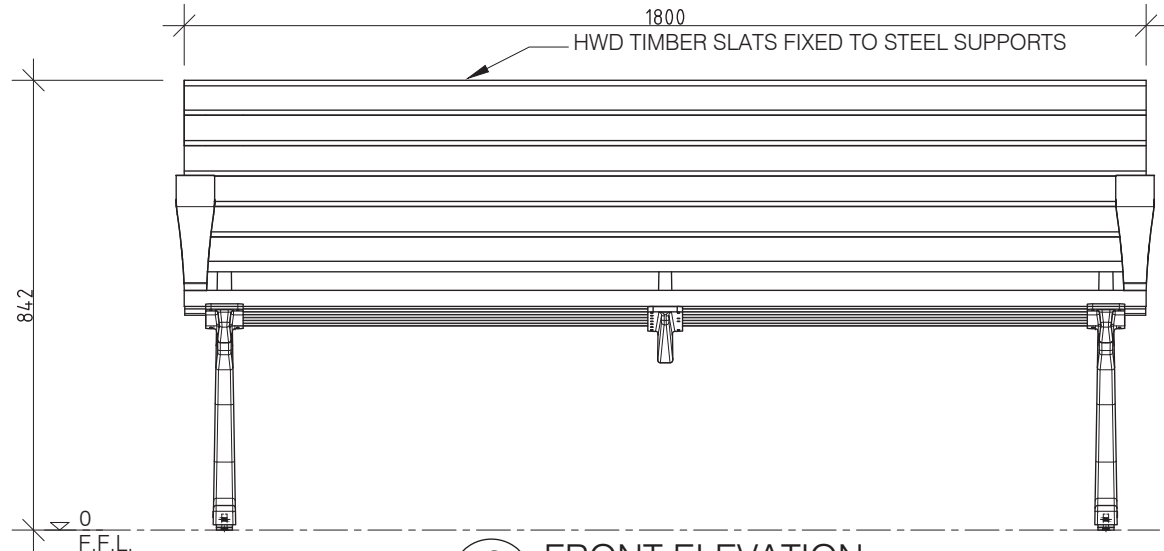
3 FRONT ELEVATION 1:10 @ A3
