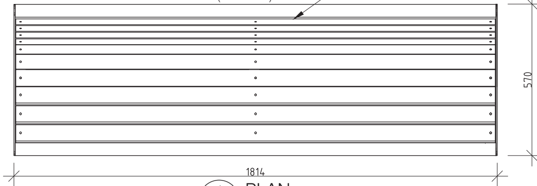
1 PLAN 1:10 @ A3 1150
