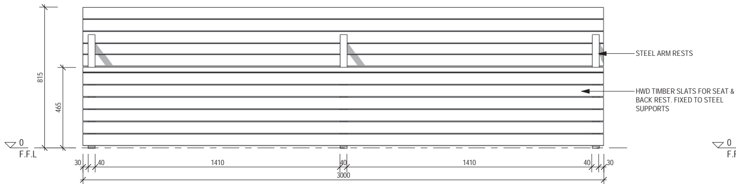
3 FRONT ELEVATION 1:15 @ A3
