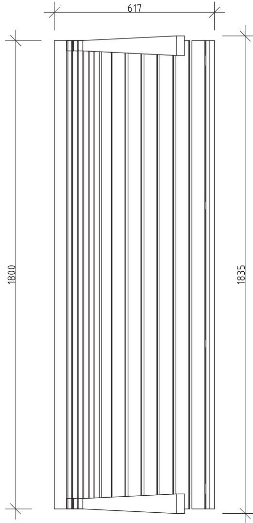
1 PLAN 1:10 @ A3
