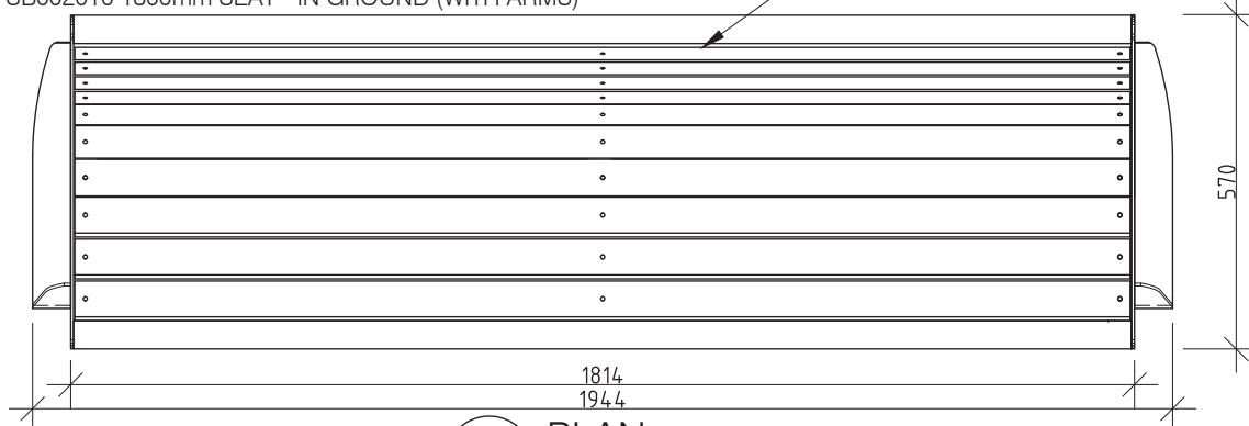
1 PLAN 1:10 @ A3
