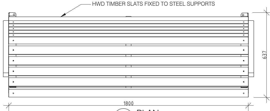
1 PLAN 1:10 @ A3
