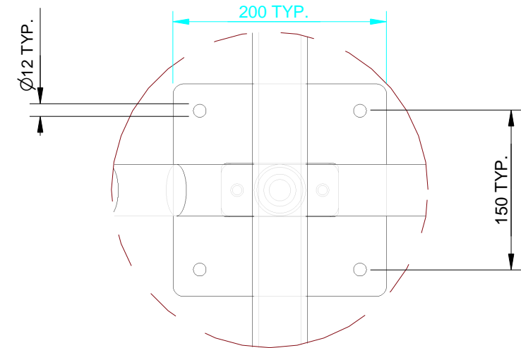
Detail A SLATS REMOVED FOR CLARITY
