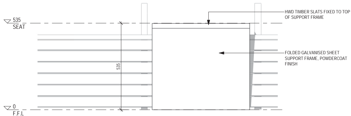
3 FRONT ELEVATION 1:10 @ A3
