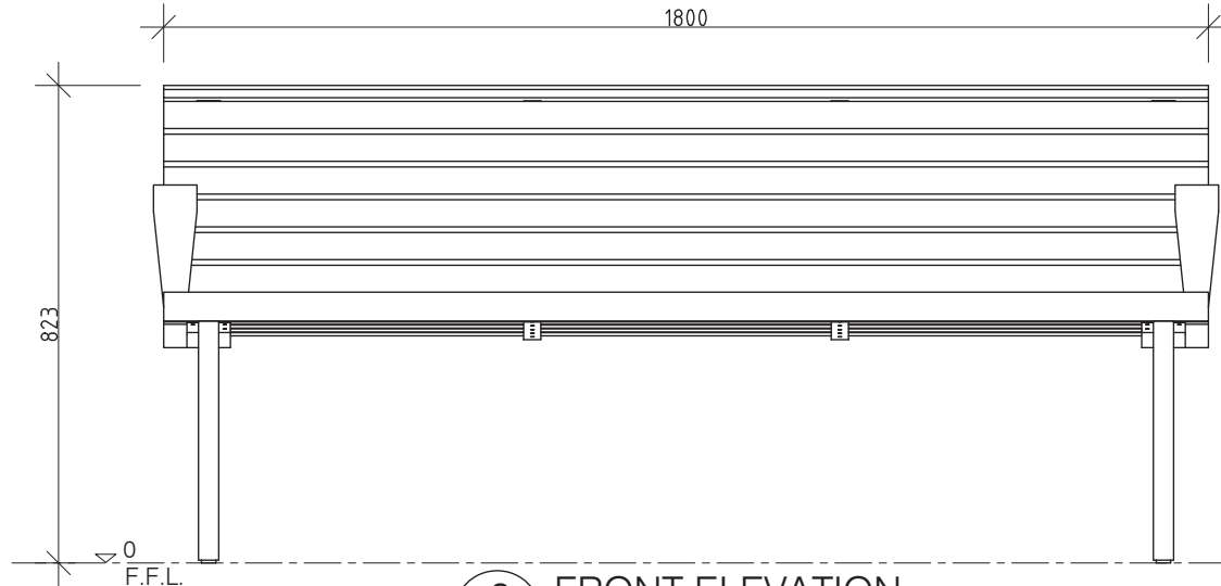
3 FRONT ELEVATION 1:10 @ A3
