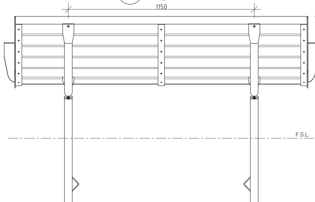
2 REAR ELEVATION 1:10 @ A3
