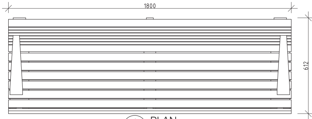
1 PLAN 1:10 @ A3
