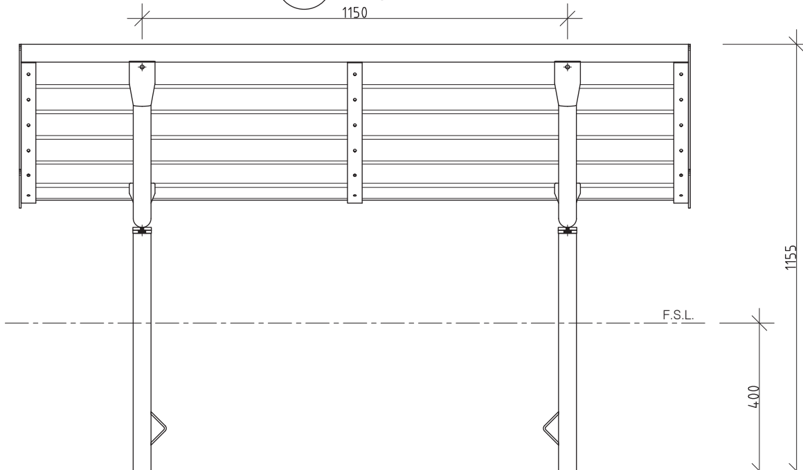
2 REAR ELEVATION 1:10 @ A3
