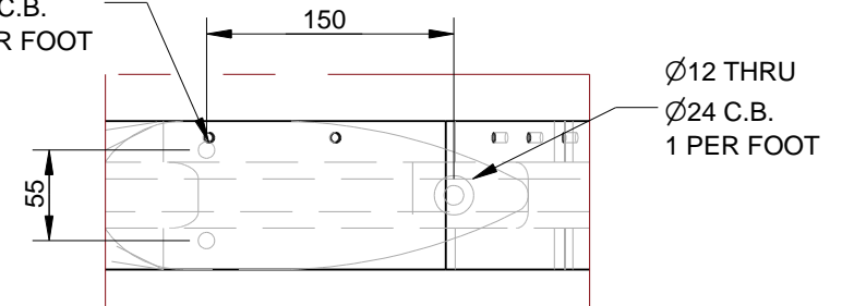
Detail A BOLT DOWN DETAIL TIMBERS AND ARM REST REMOVED FOR CLARRITY
