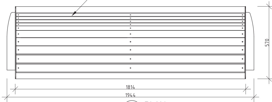
1 PLAN 1:10 @ A3
