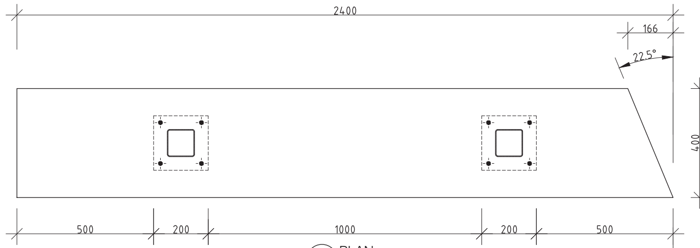
1 PLAN 1:10 @ A3
