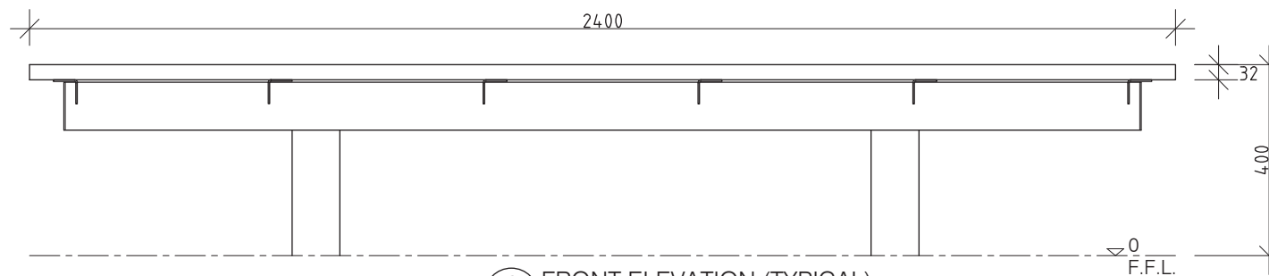
2 FRONT ELEVATION (TYPICAL) 1:10 @ A3
