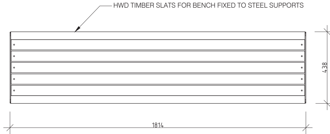
1 PLAN 1:10 @ A3
