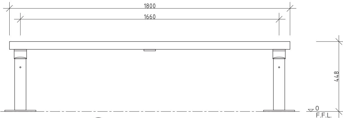
2 FRONT ELEVATION 1:10 @ A3
