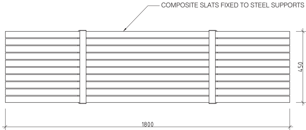
1 PLAN 1:10 @ A3
