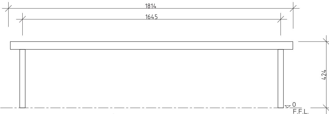
2 FRONT ELEVATION 1:10 @ A3
