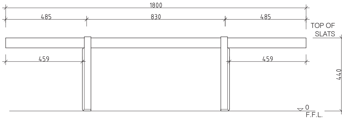
2 FRONT ELEVATION 1:10 @ A3
