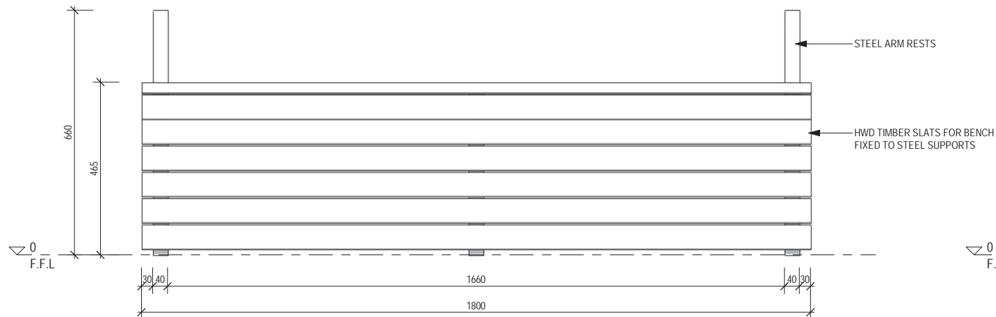
3 FRONT ELEVATION
