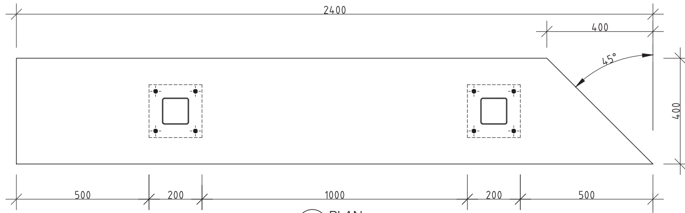
1 PLAN 1:10 @ A3
