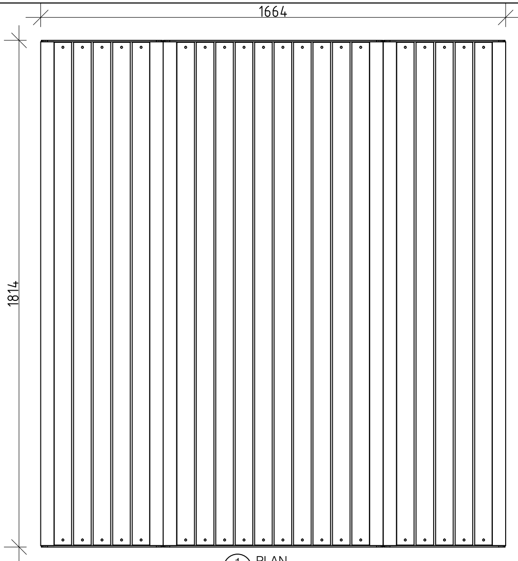
1 PLAN 1:15 @ A3
