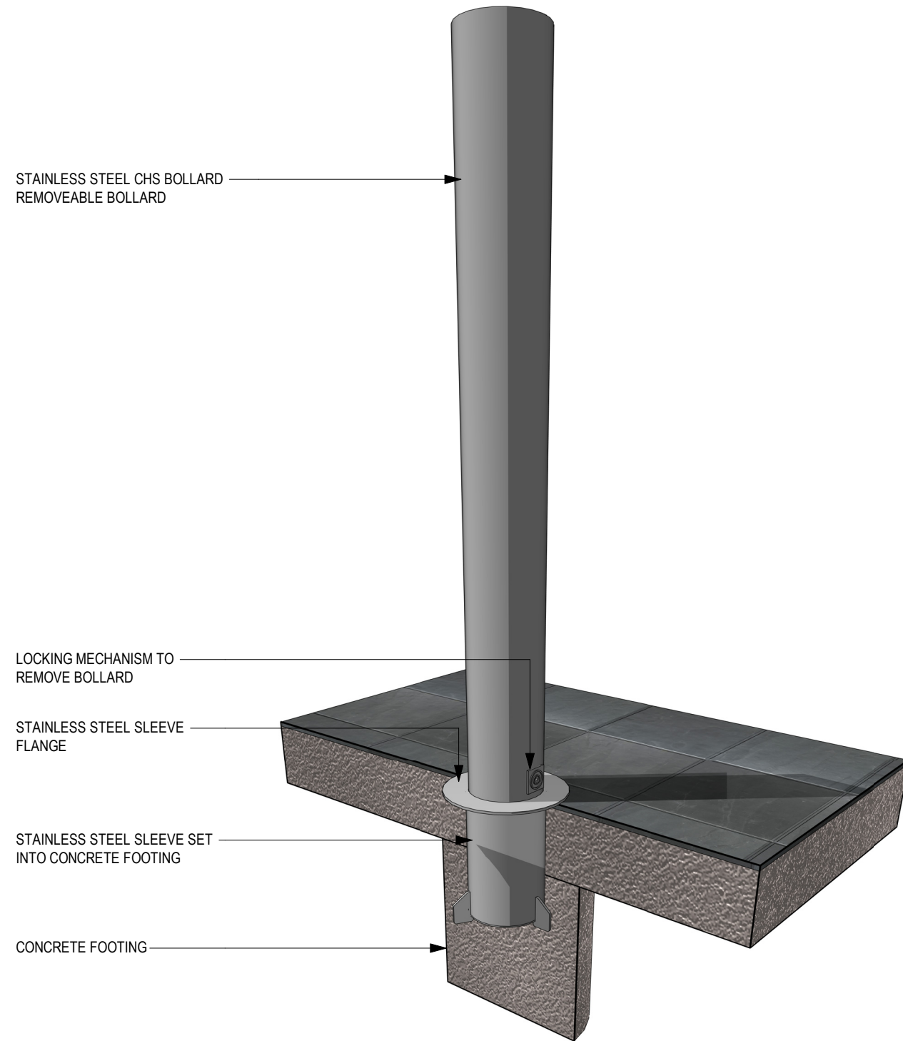
4 SECTIONAL PERSPECTIVE @ A3
